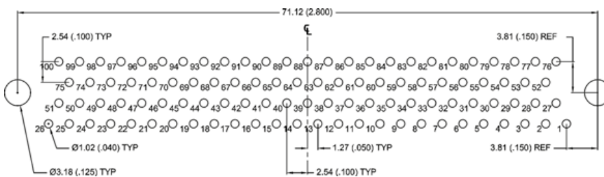
100 CONTACTS - VIEW A
