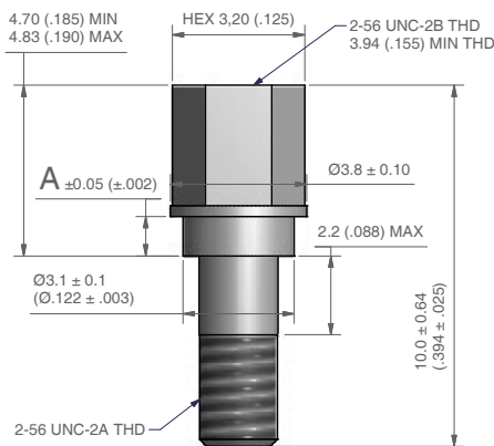
KIT PART NUMBER: MDAHMSP0x Hardware code: Px
