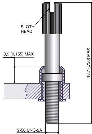
HARDWARE CODE: K
