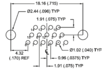
15 CONTACTS - VIEW A
